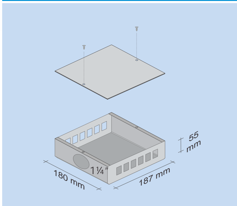
CCPE18R 1 1/4"
